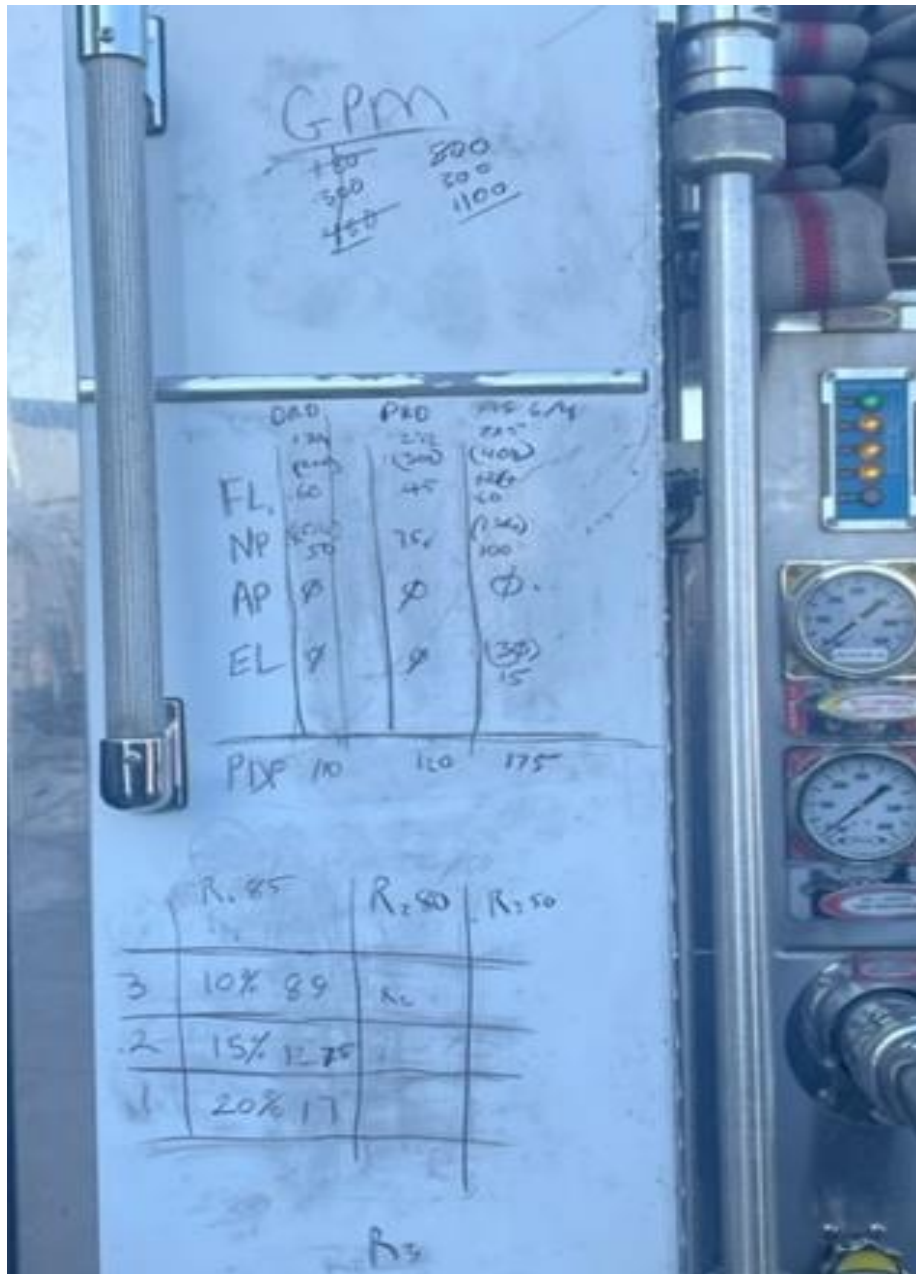
Figure 10: An example of using a grease pencil to keep track of calculations on the side of the rig next to the pump panel
